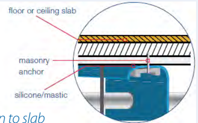
Installation to slab
